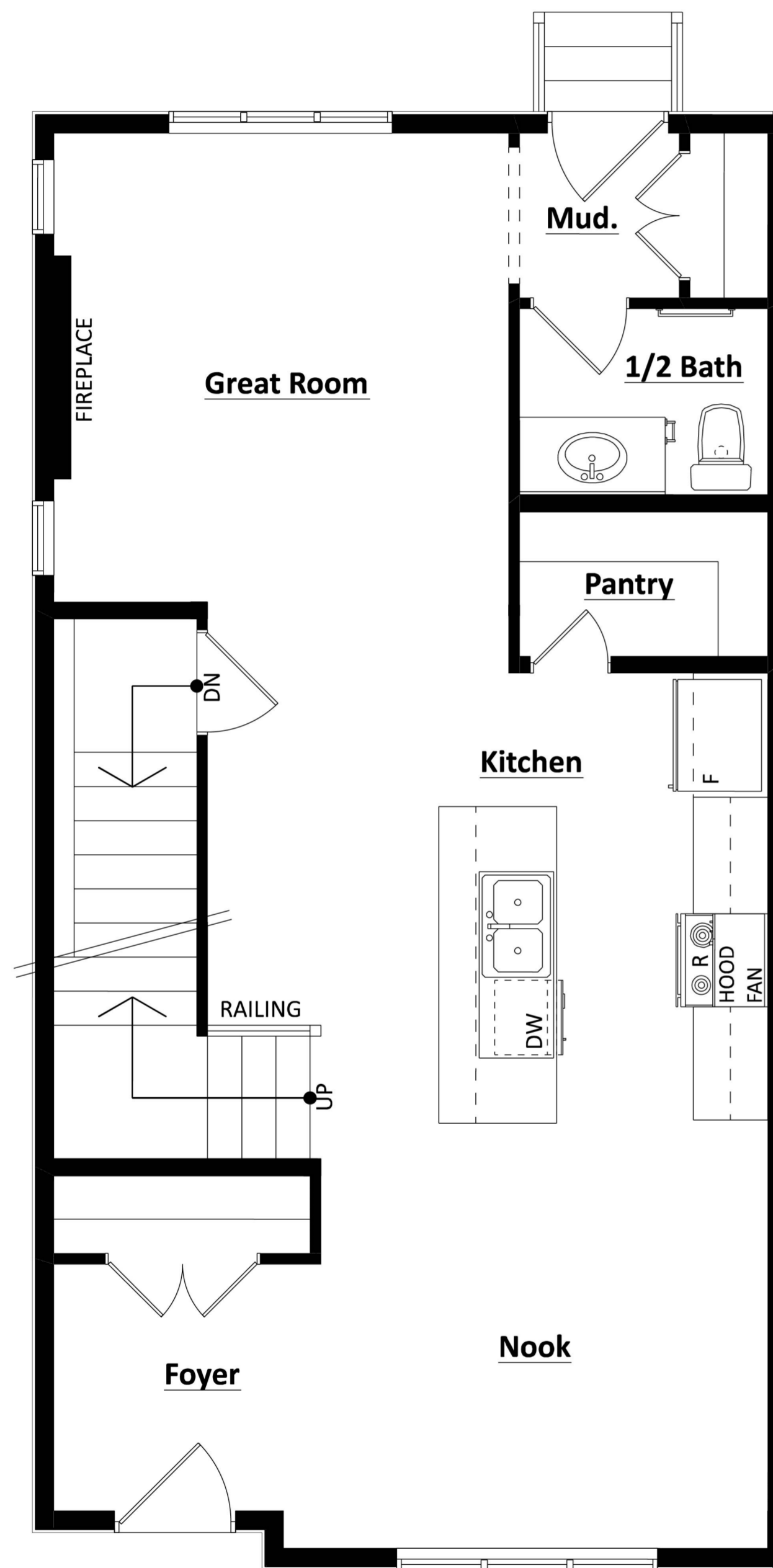
Unit 1- Main Floor Plan
