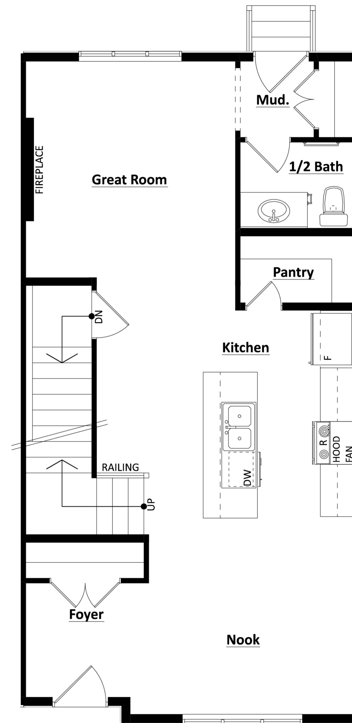
Unit 3- Main Floor Plan
