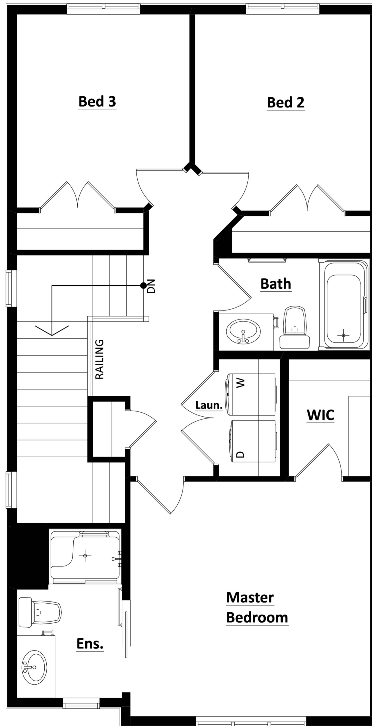
Unit 1- Second Floor Plan
